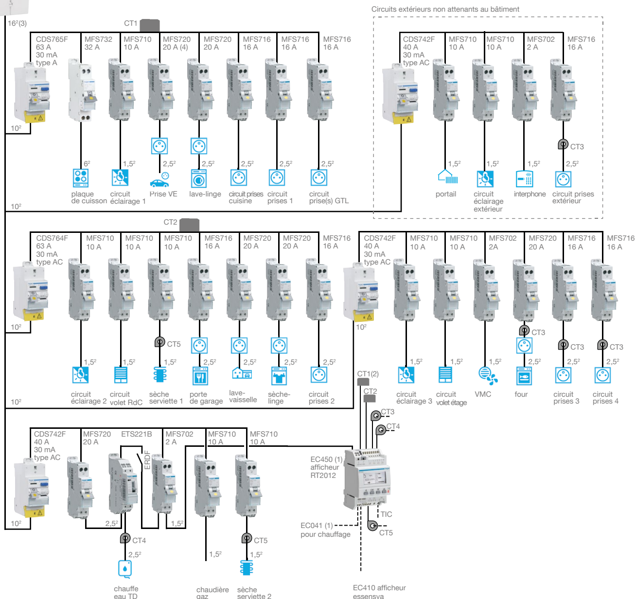
HDA260SF DB In 60 A 12 kVA individuel 500 mA type S
